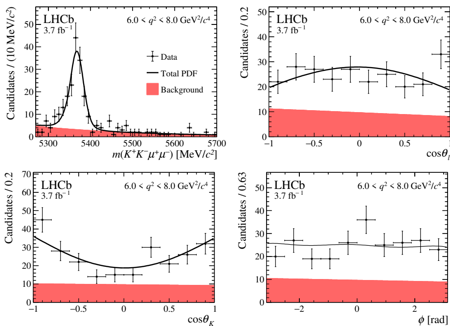
Figure 23. Mass and angular distributions of B_s^0 \rightarrow \phi\mu^+\mu^- candidates in the region 6.0 < q^2 < 8.0 \text{ GeV}^2/c^4 for data taken in 2017–2018. The data are overlaid with the projections of the fitted PDF.
