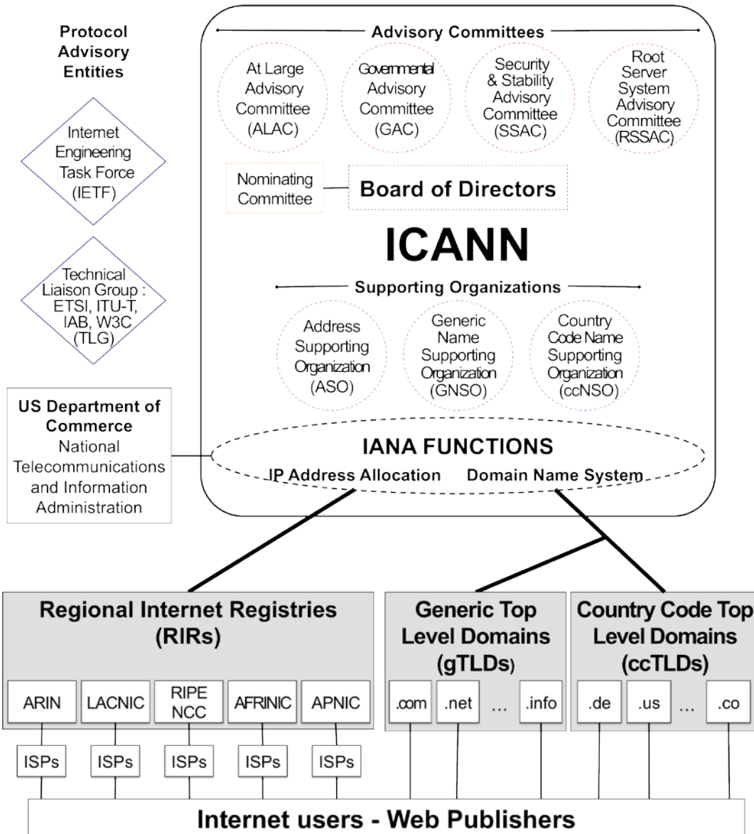
Figure 5: ICANN structure.
