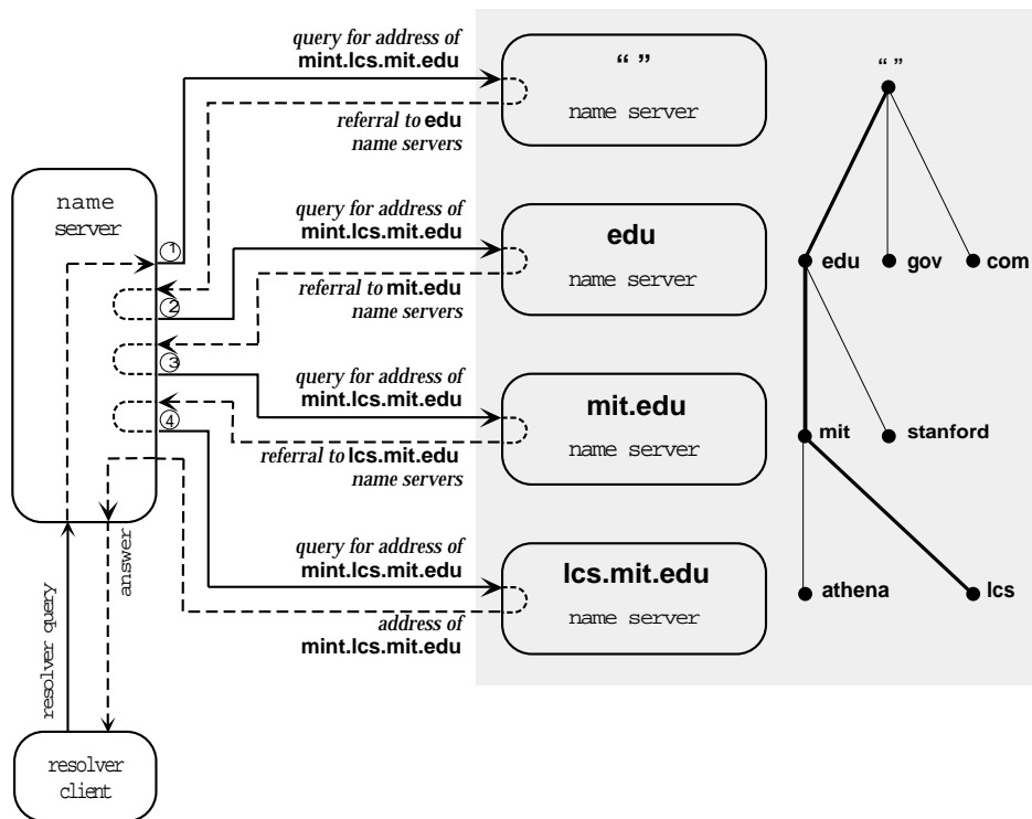
Figure 2.2: Recursive queries 1
