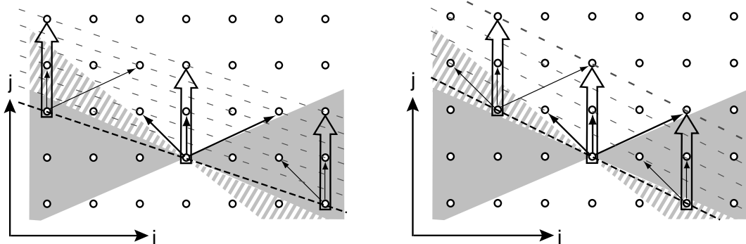
Figure 4: Iteration space diagram for Example 1. Given an occupancy vector of (0, 2) , our method identifies the range of valid schedules. An affine schedule will sweep across the space, executing a line of iterations at once. If this line falls within the gray region (as on the left), then the schedule is valid for the occupancy vector. If this line falls within the striped region (as on the right) then the schedule is invalid because of the parallel read/write occurring from the tip of the occupancy vector.
