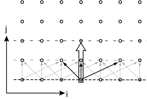
Figure 2: Iteration space diagram for Example 1. Given the schedule where each row is executed in parallel, our method identifies (0, 2) as the shortest valid occupancy vector.
