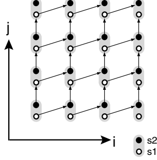
Figure 8: Dependence diagram for Example 2.
