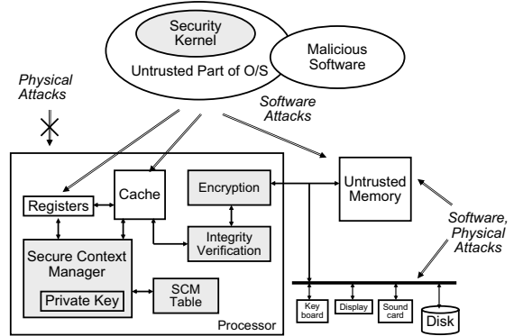
Figure 1: Our secure computing model.
