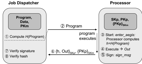
Figure 4: Certified execution for distributed computation.
