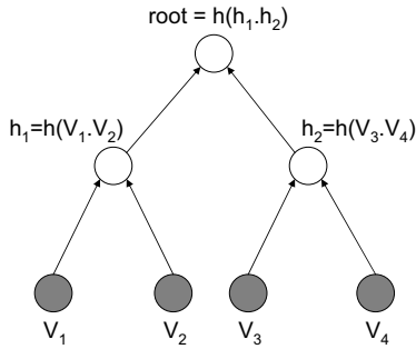
Figure 2: A binary hash tree. Each internal node is a hash of the concatenation of the data in the node’s children.
