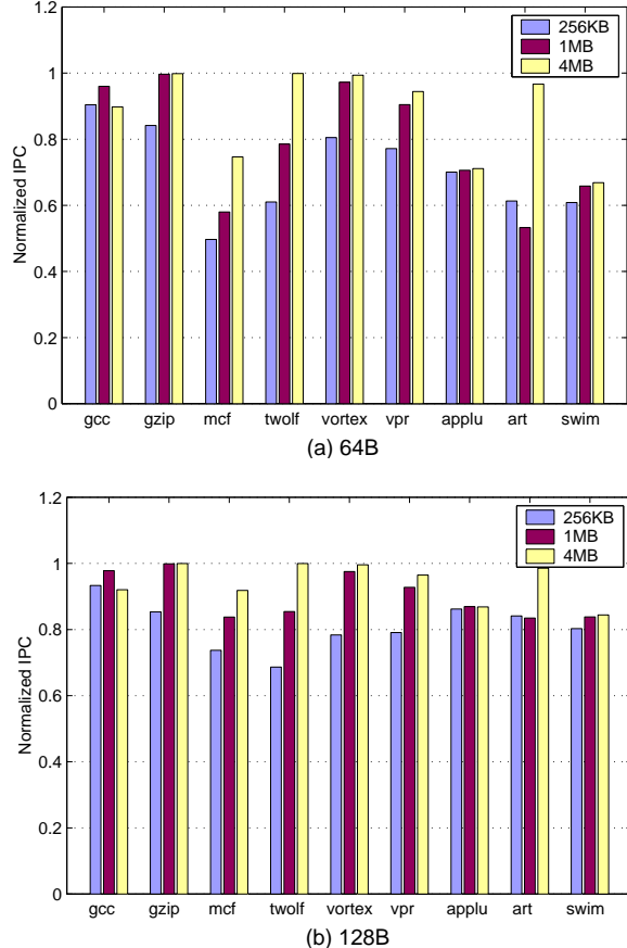
Figure 6: The performance overhead of TE processing. The results are shown for various L2 cache sizes with two block sizes (64B and 128B).
