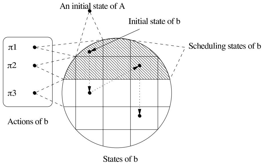
Fig. 4. The execution of some automaton b \in \mathcal{B} .
