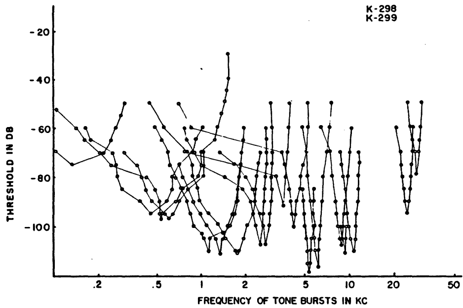
Figure 2.3: Physiological Tuning Curves obtained by combining the data from two cats. [from Kiang et al. 1965].
