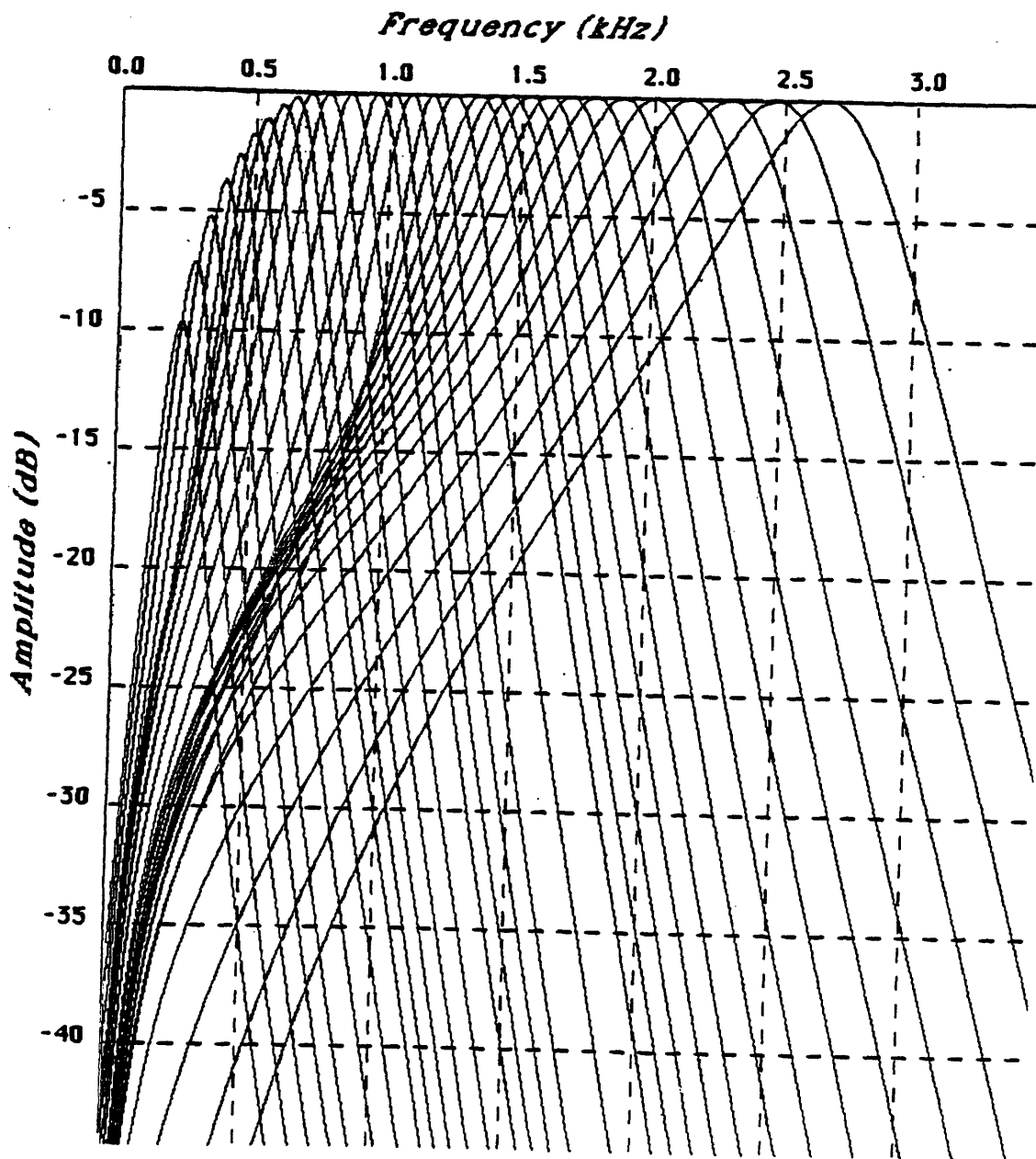
Figure 11.5: b) Filter characteristics used for Figures 11.4, Part (iii). The filters centered above about 1000 Hz have broader low frequency tails than in Part (a).
