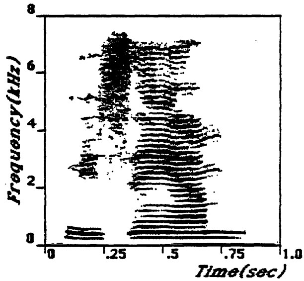
Figure 12.2: Comparison of narrow-band spectrograms [25 ms Hamming window] for pitch waveform versus original waveform for the word "museum", spoken by a female speaker.
