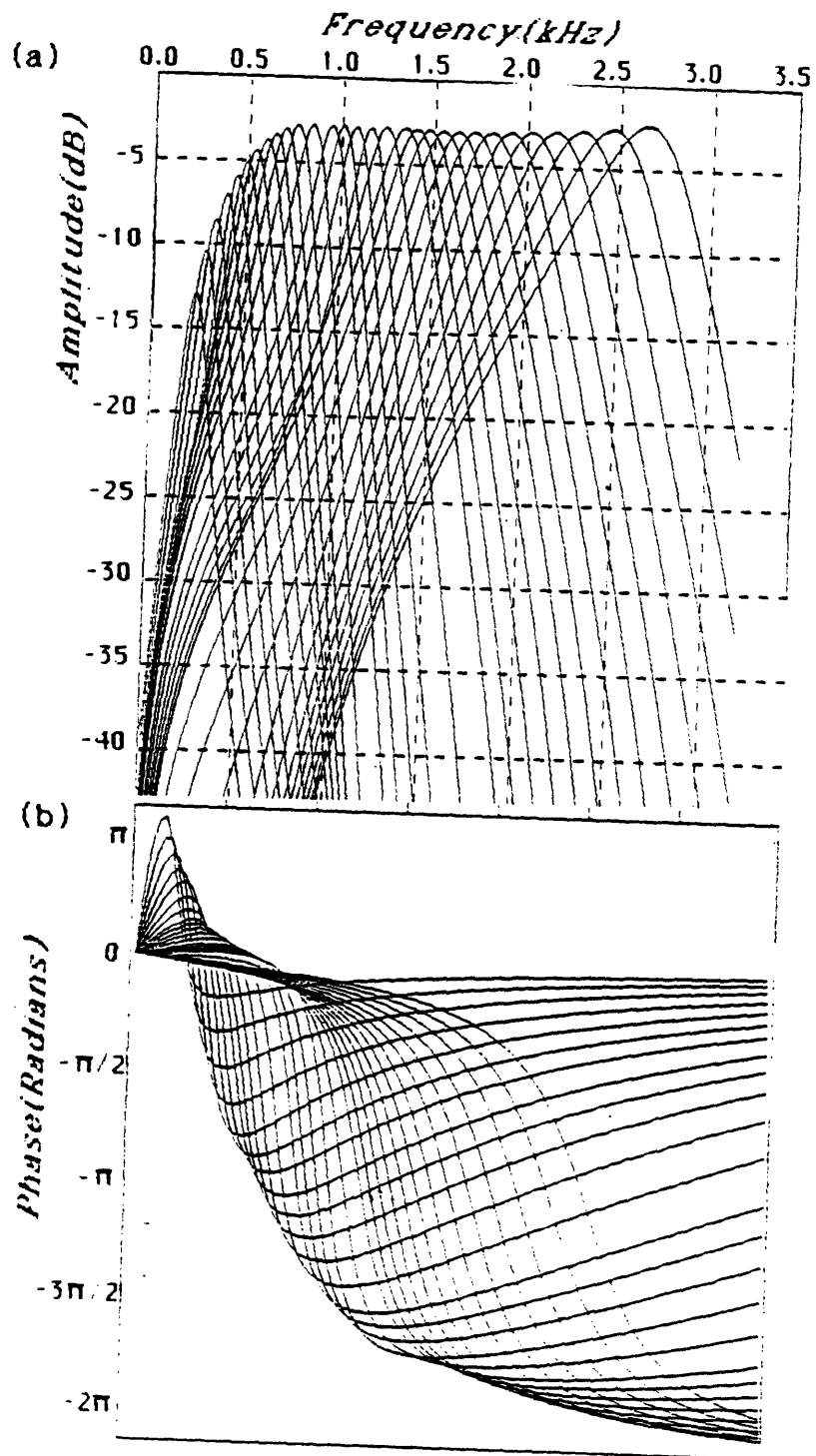
Figure 8.2: Magnitude (a) and phase (b) response characteristics of bank of 30 filters used to model auditory filters. Linear phase term has been removed.
