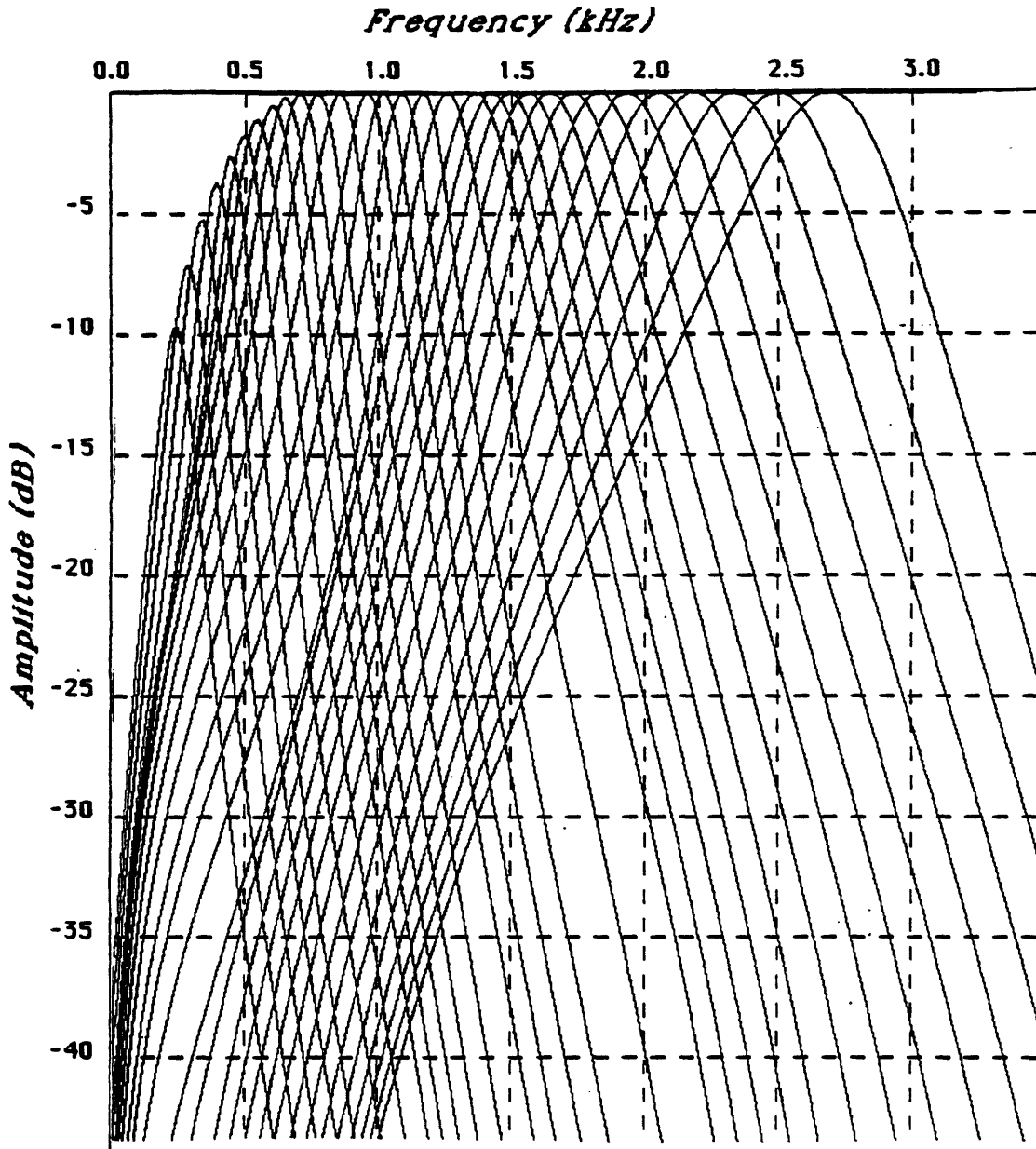
Figure 11.5: Filter characteristics for systems illustrated in Figure 11.4, Parts (ii), (iii), and (iv), to show effect of broader filters on synchrony measure.
