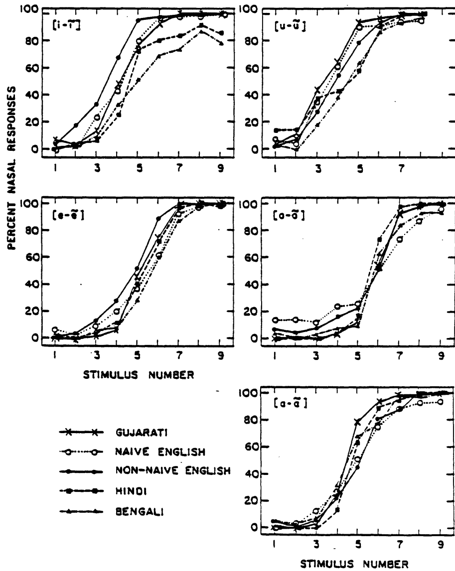
Figure 10.12: Results of a perceptual study of the vowel stimuli described in Figure 10.11. Each subject was asked to identify each stimulus as nasalized or non-nasalized. The data are separated into five distinct subject classes. Each vowel series shows a consistent trend towards increased nasalization with increased separation of the pole-zero-pole complex in the first formant frequency region. [From Hawkins and Stevens, in press.]
