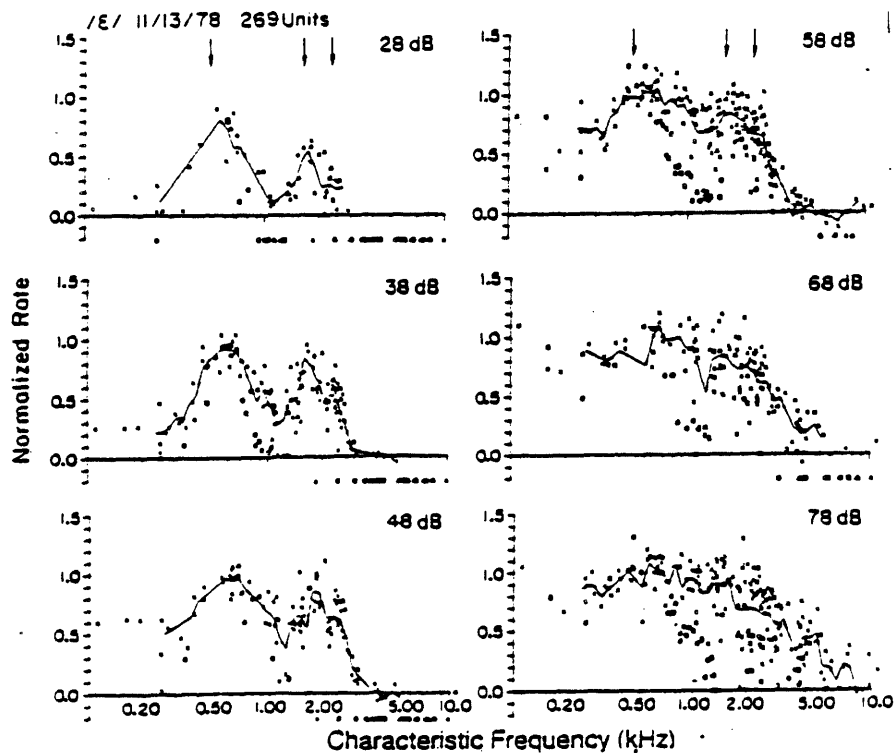
Figure 2.6: Normalized rate vs CF for 260 units studies on 11/13/78 with synthesized /ε/ as the stimulus. Positions of the formant frequencies are shown by the arrows. [from Sachs and Young, 1979].
