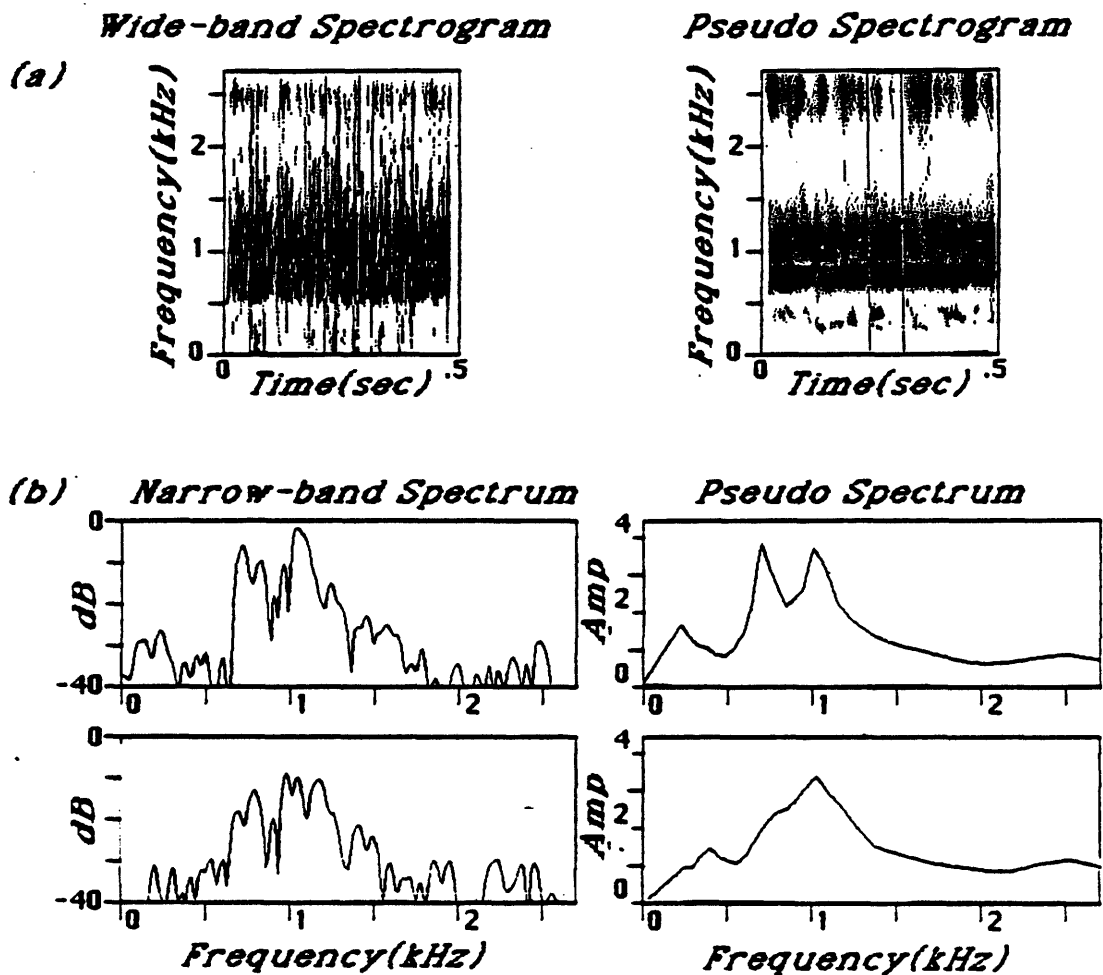
Figure 10.4: Example of pseudo-spectral analysis of noise-excited synthetic speech, with formant frequencies at 700 and 1050 Hz.
