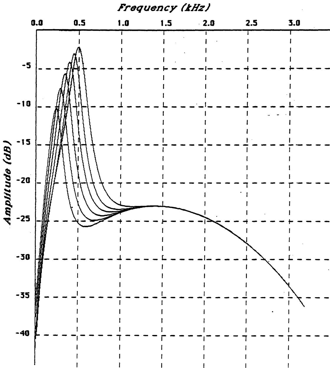
Figure 9.16: Filter characteristics of low frequency filters used for part (c) of Figure 9.9.
