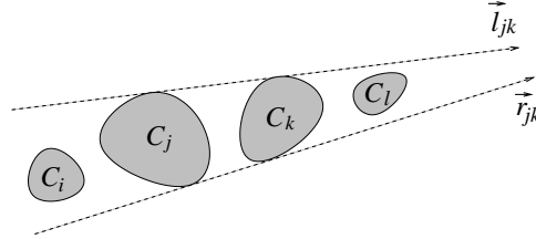
Figure 2: For Lemma 7.7.
