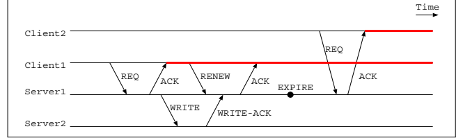
Fig. 6. Duplicated lease scenario for the mutated DHCP-F
